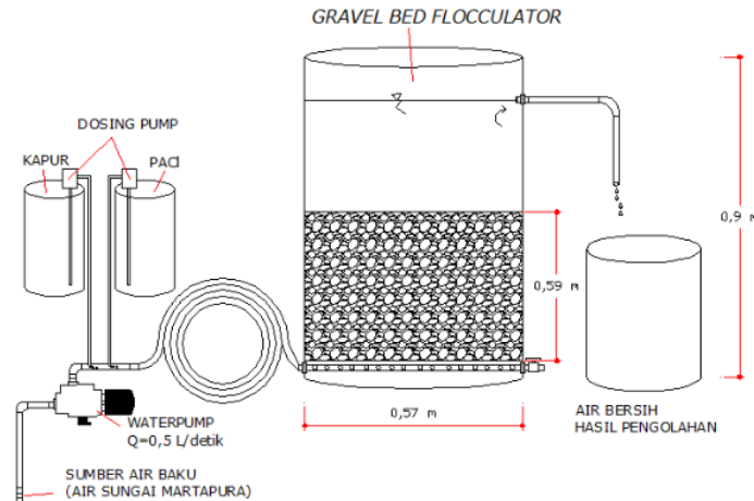
Gambar 1. Sketsa Gravel Bed Flocculator
